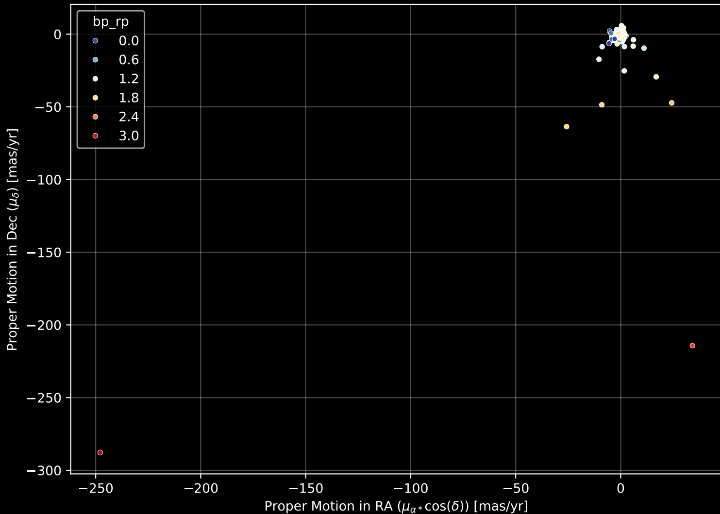
APOGEE DR17 Field: [206+04] Proper Motion Diagram (n= 181)
