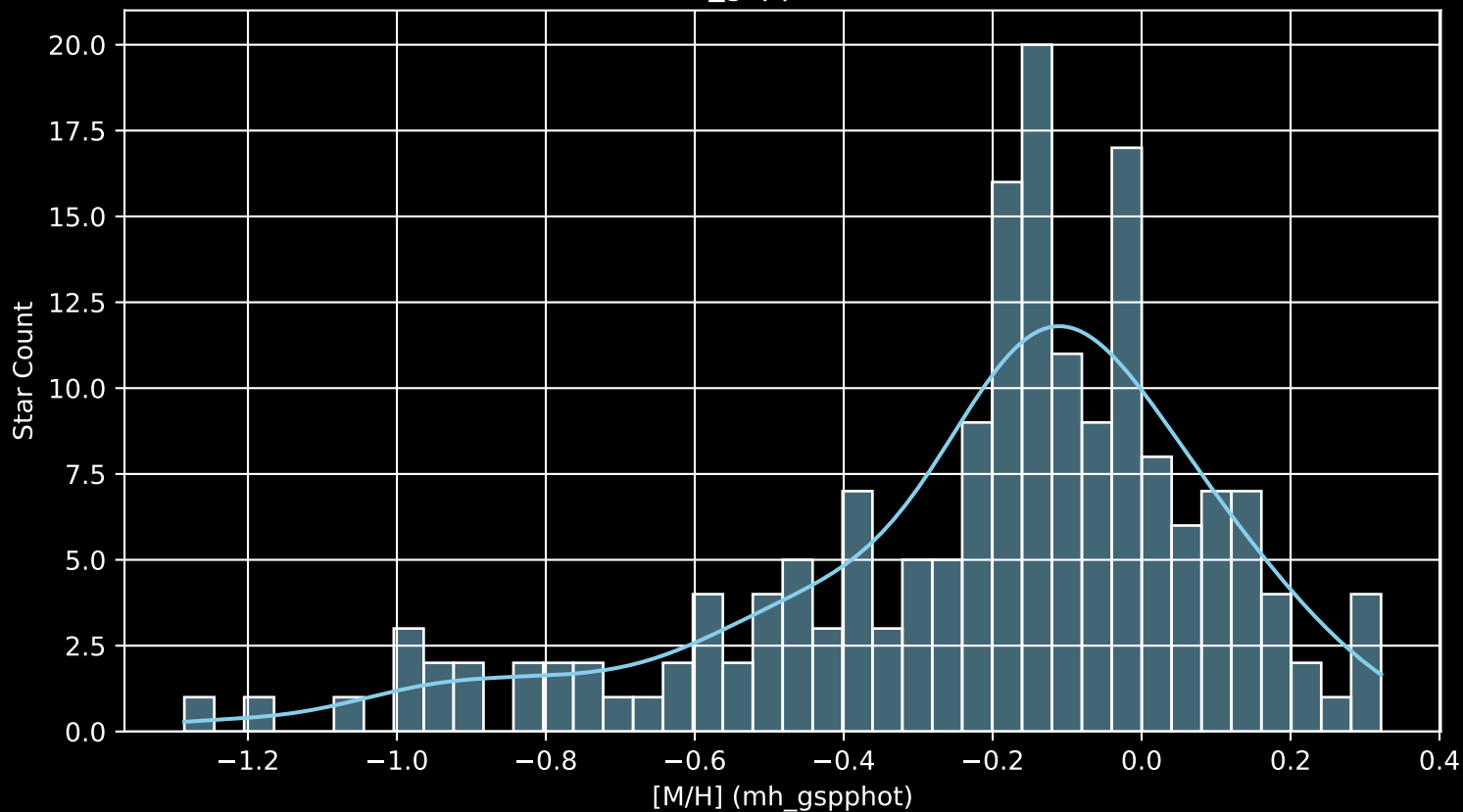
APOGEE DR17 Field: [206+04 [M/H] (mh_gspphot) (n= 179)
